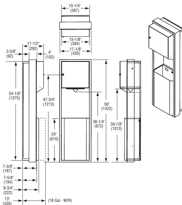
Semi-Recessed
