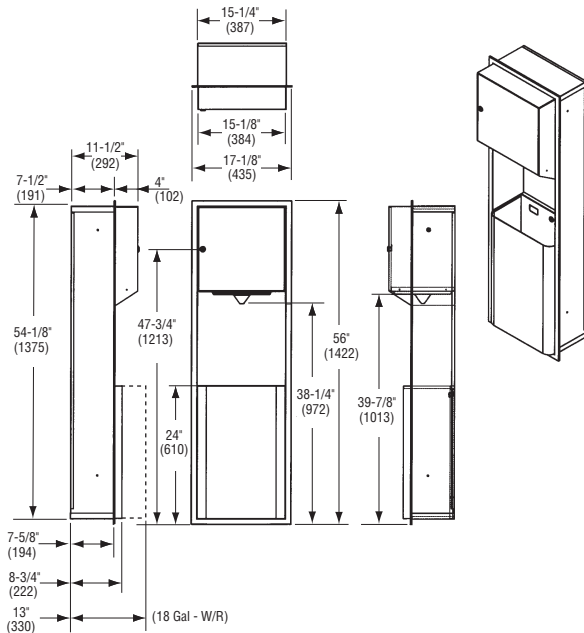
Recess-Mounted
